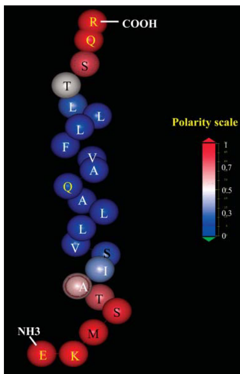
FIGURE 7 The average position of M26 in the lipid bilayer in the TM orientation. In the simulations, each residue in the peptide was represented by two interaction centers (backbone and side chain). Here, each residue is presented as a single sphere, for clarity. The spheres are located at the C^\alpha nuclei. The identities of the residues are noted by one letter code. The peptide is colored according to the polarity of the environment of each residue in the average position. The color code appears in the scale at the right side of the figure.
